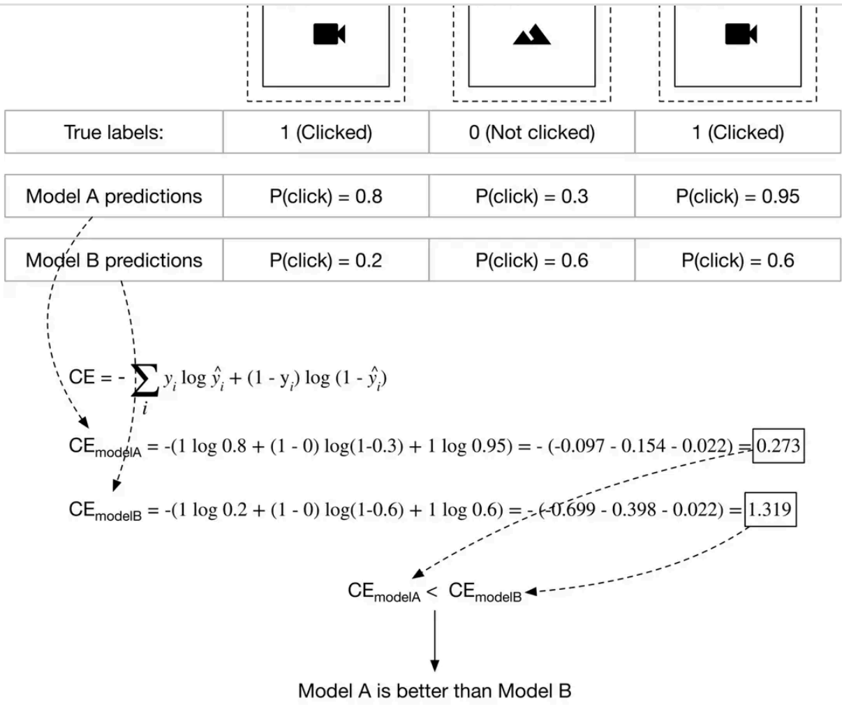
Figure 8.16: CE of two ML models
