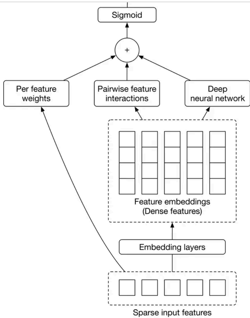
Figure 8.14: DeepFM overview
