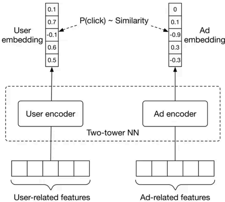
Figure 8.11: Embedding-based NN
