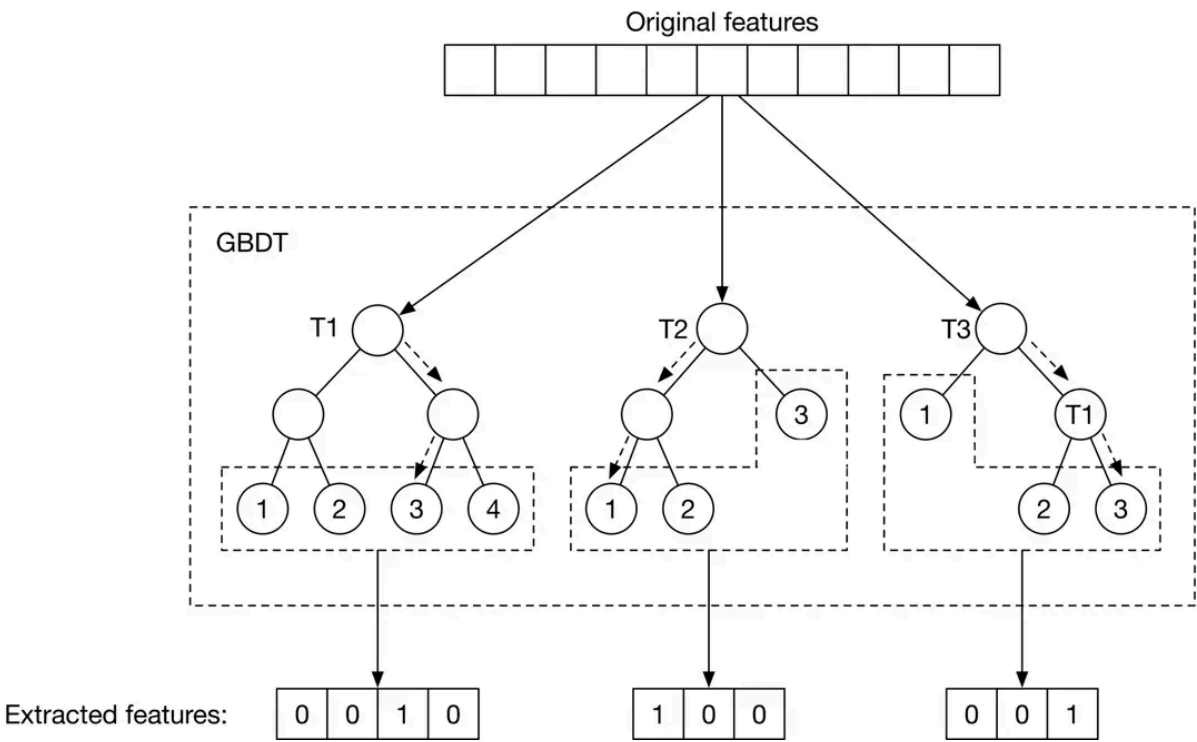
Figure 8.8: Use GBDT for feature extraction
