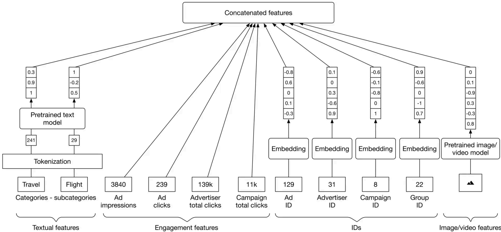
Figure 8.4: Summary of ad-related feature preparation
