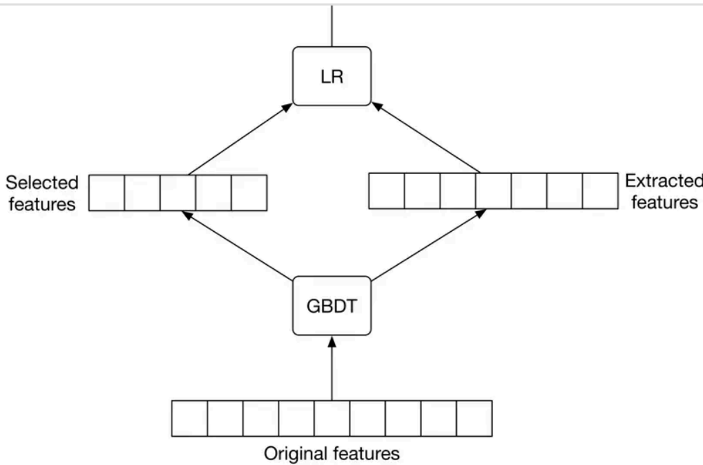
Figure 8.9: GBDT + LR overview
