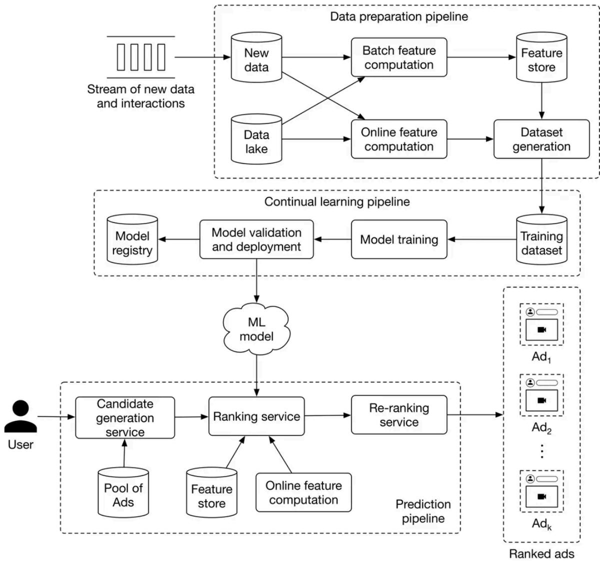
Figure 8.18: ML system design
