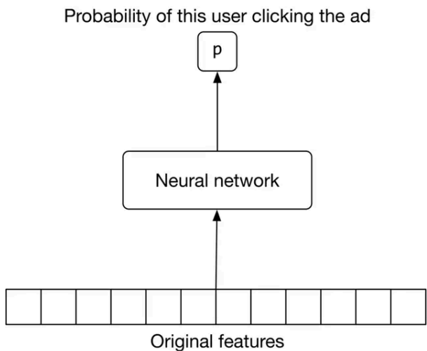
Figure 8.10: NN architecture
