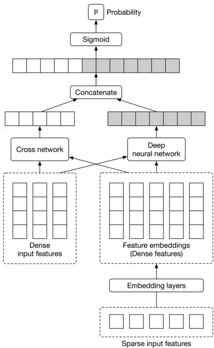
Figure 8.12: DCN architecture
