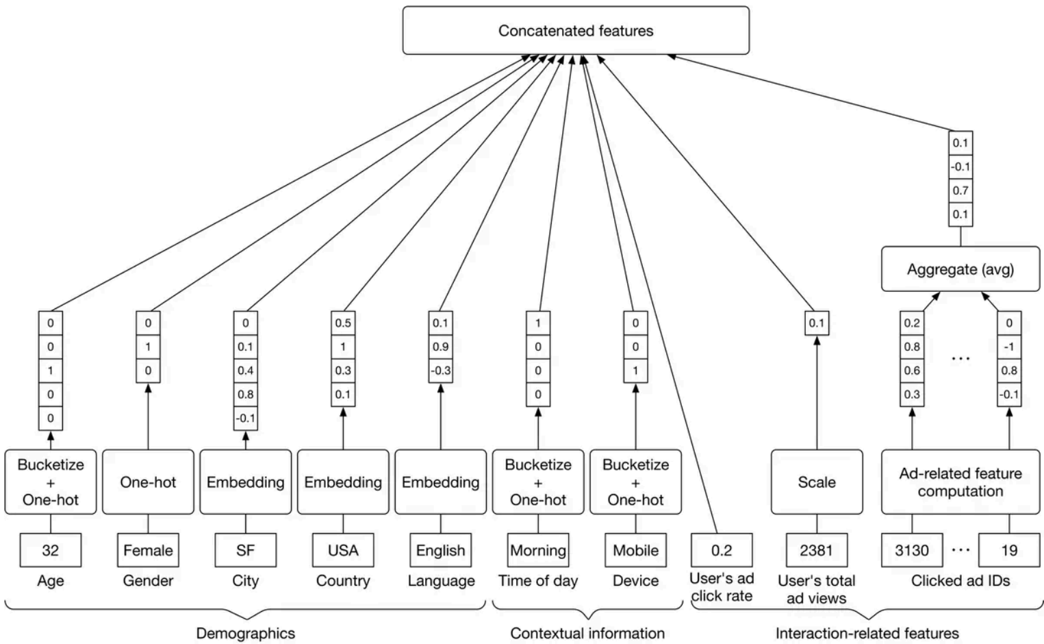
Figure 8.5: Feature preparation for user metadata and interactions
