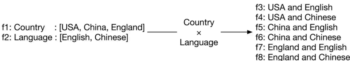
Figure 8.6: Crossing two features: country and language
