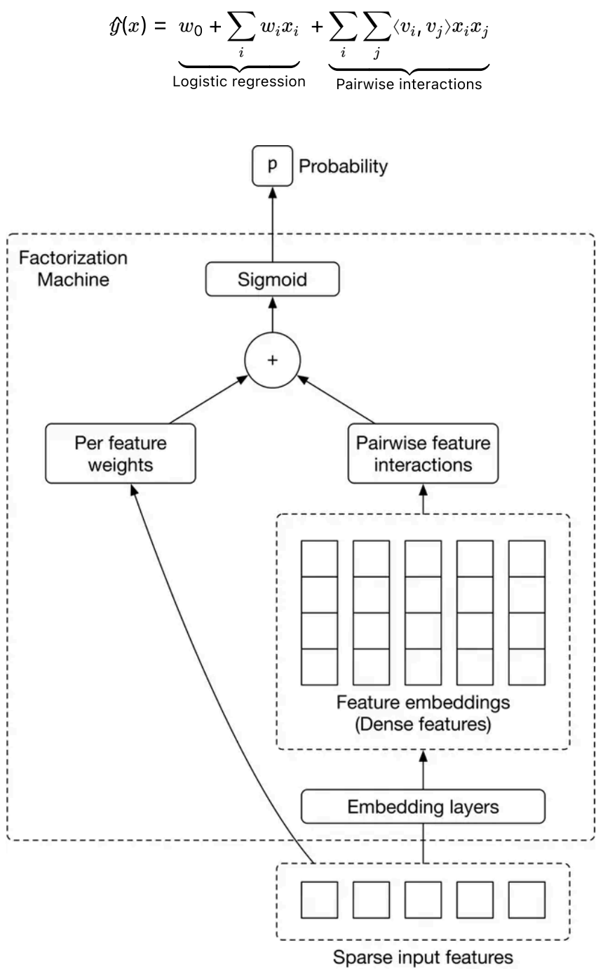
Figure 8.13: Factorization Machine architecture
